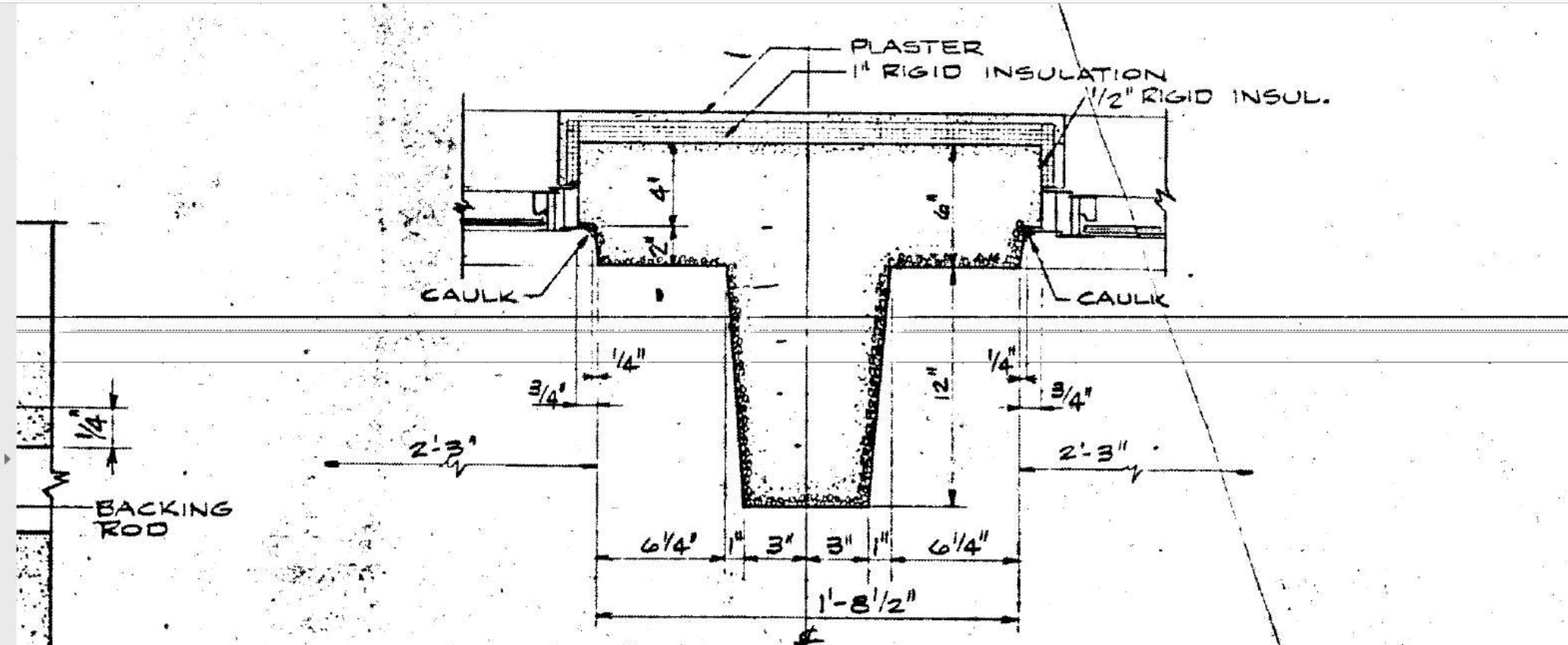
2 TYP. FIN DETAIL 8.1 SCALE: 1 1/2" = 1'-0"
