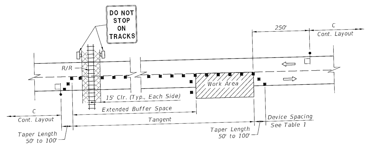
LAYOUT FOR RAILROAD CROSSING BUFFER SPACE EXTENSION
